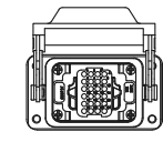
X2 SIGNAL CONNECTOR MENCOM CDDF-24 44mm x 27mm (6B) 24P 10A FEMALE
