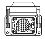
X1 SIGNAL PLUG MENCOM CDDM-24 44mm x 27mm (6B) 24P 10A MALE
