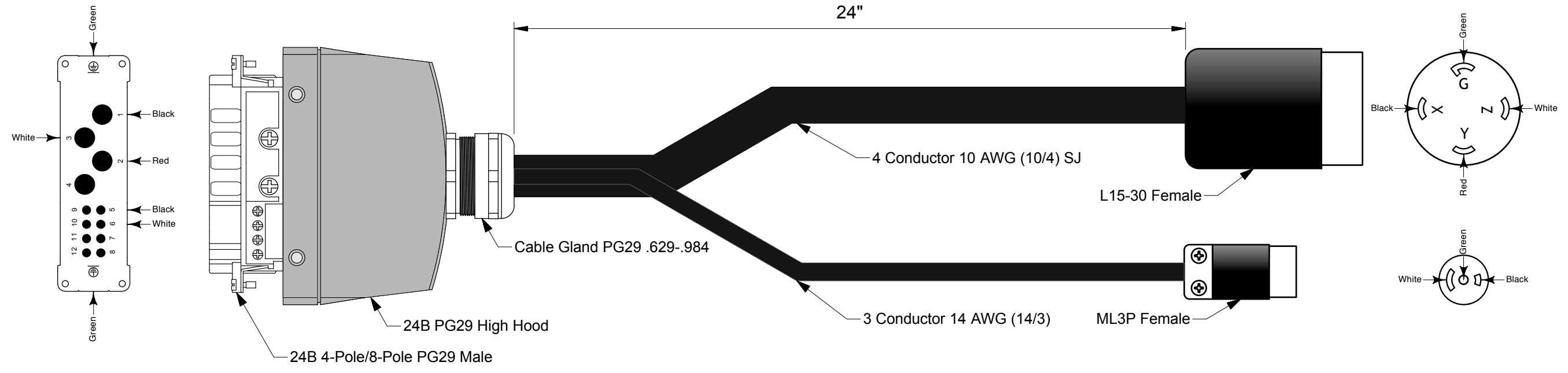
Stagehand Pro Motor Squid scale: nts
