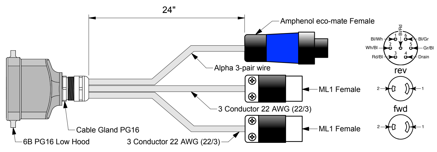
Stagehand Pro Motor Squid scale: nts
